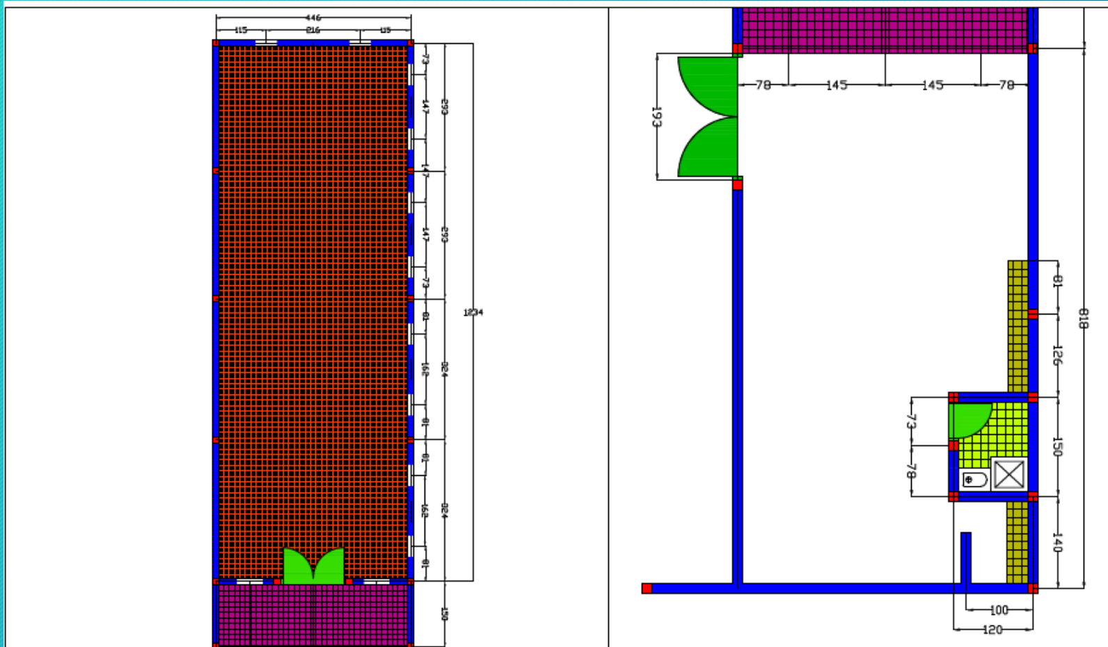
Denah
